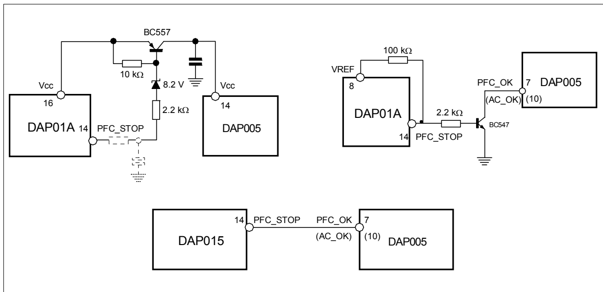
Figure 43. Interface circuits that let DC-DC converter's controller IC disable the DAP005 at light load
