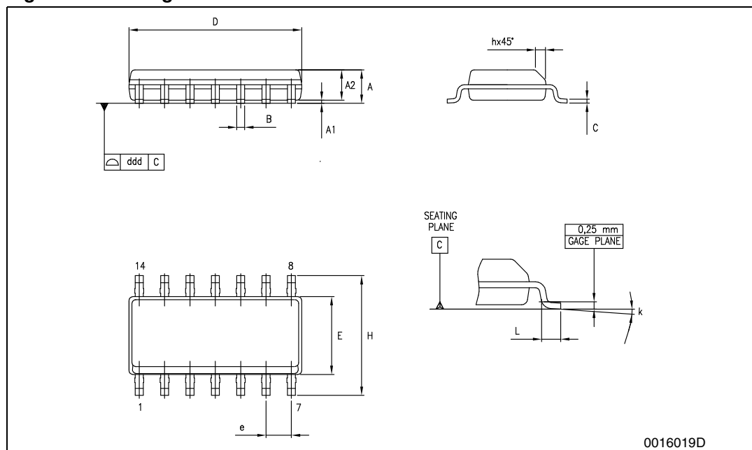
Figure 54. Package dimensions
