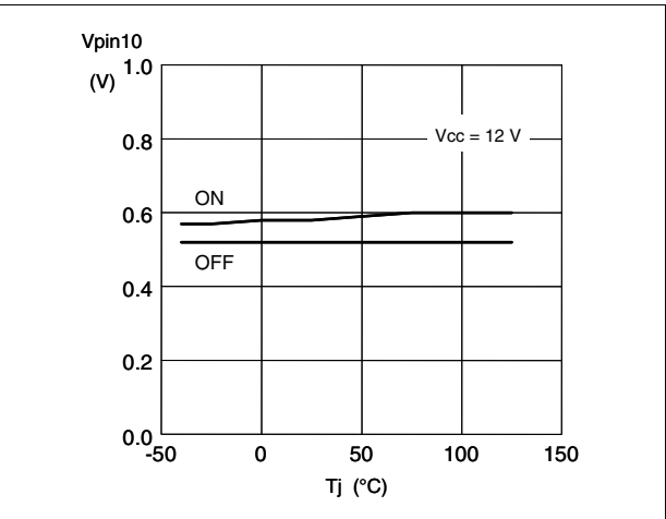
Figure 23. AC_OK thresholds vs T_J
