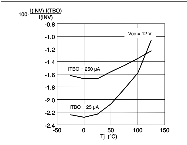
Figure 22. TBO current mismatch vs T_J
