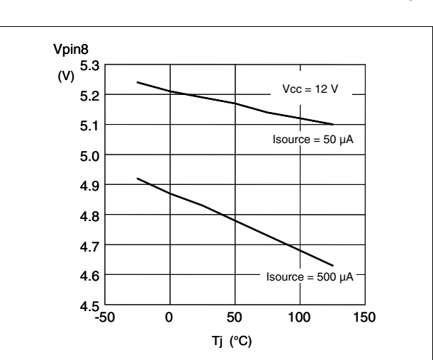
Figure 25. PWM_LATCH high saturation vs T_J
